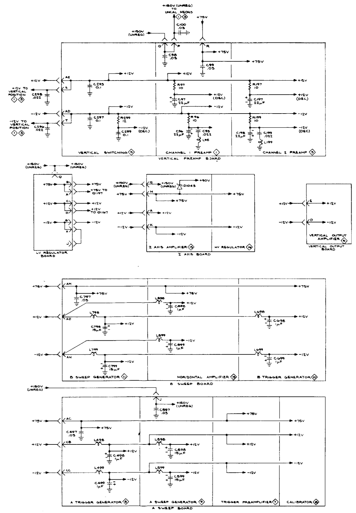
FIG. FO-27. POWER SUPPLY & DISTRIBUTION (5/N 20,000 & UP)
