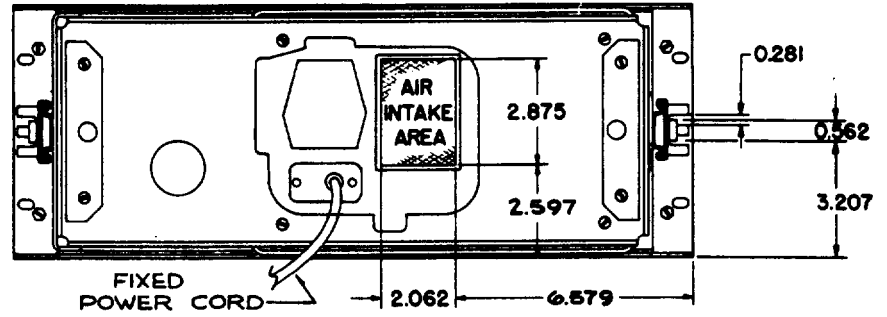
Figure 10-12. REAR VIEW
