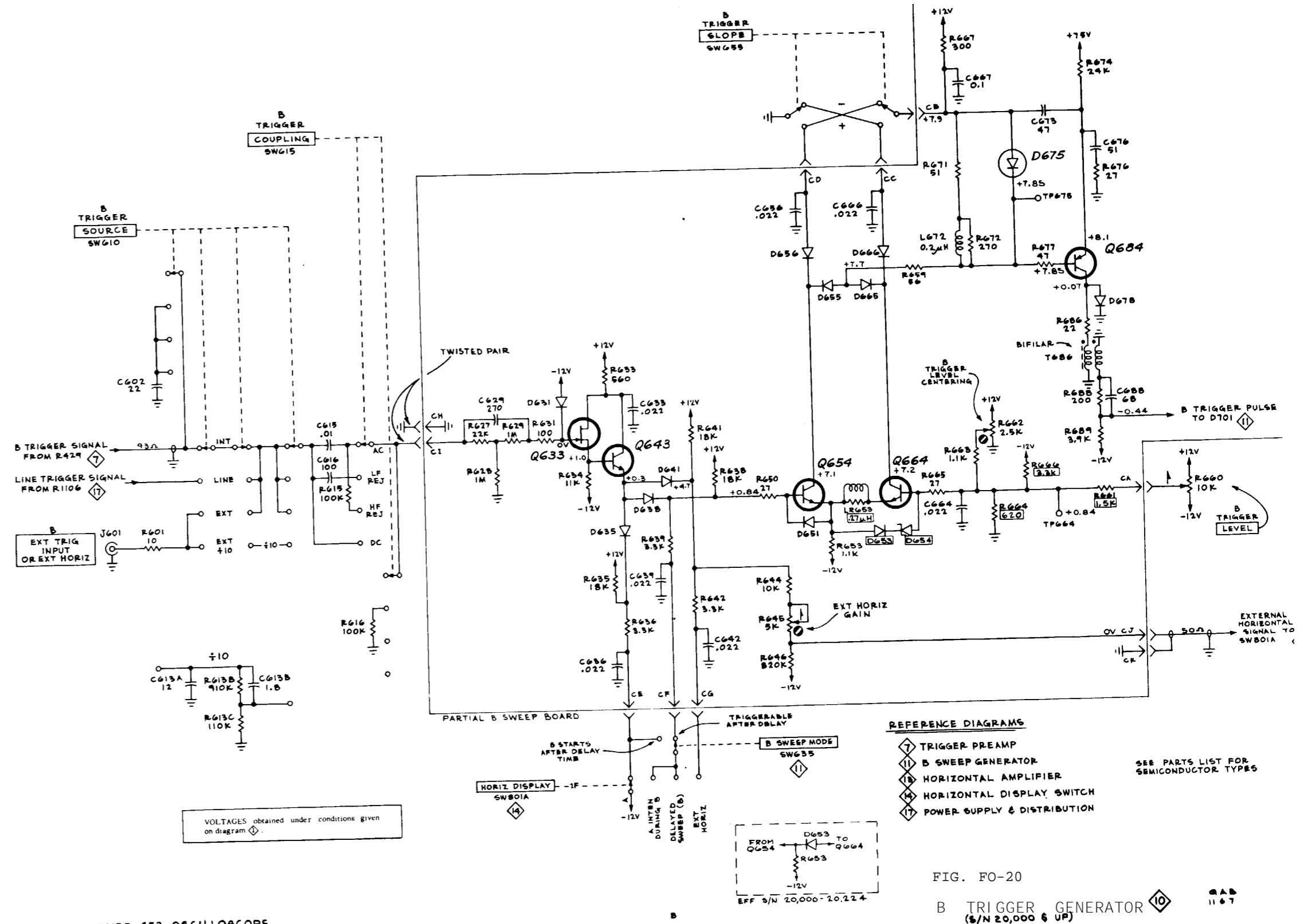
TYPE 453 OSCILLOSCOPE
