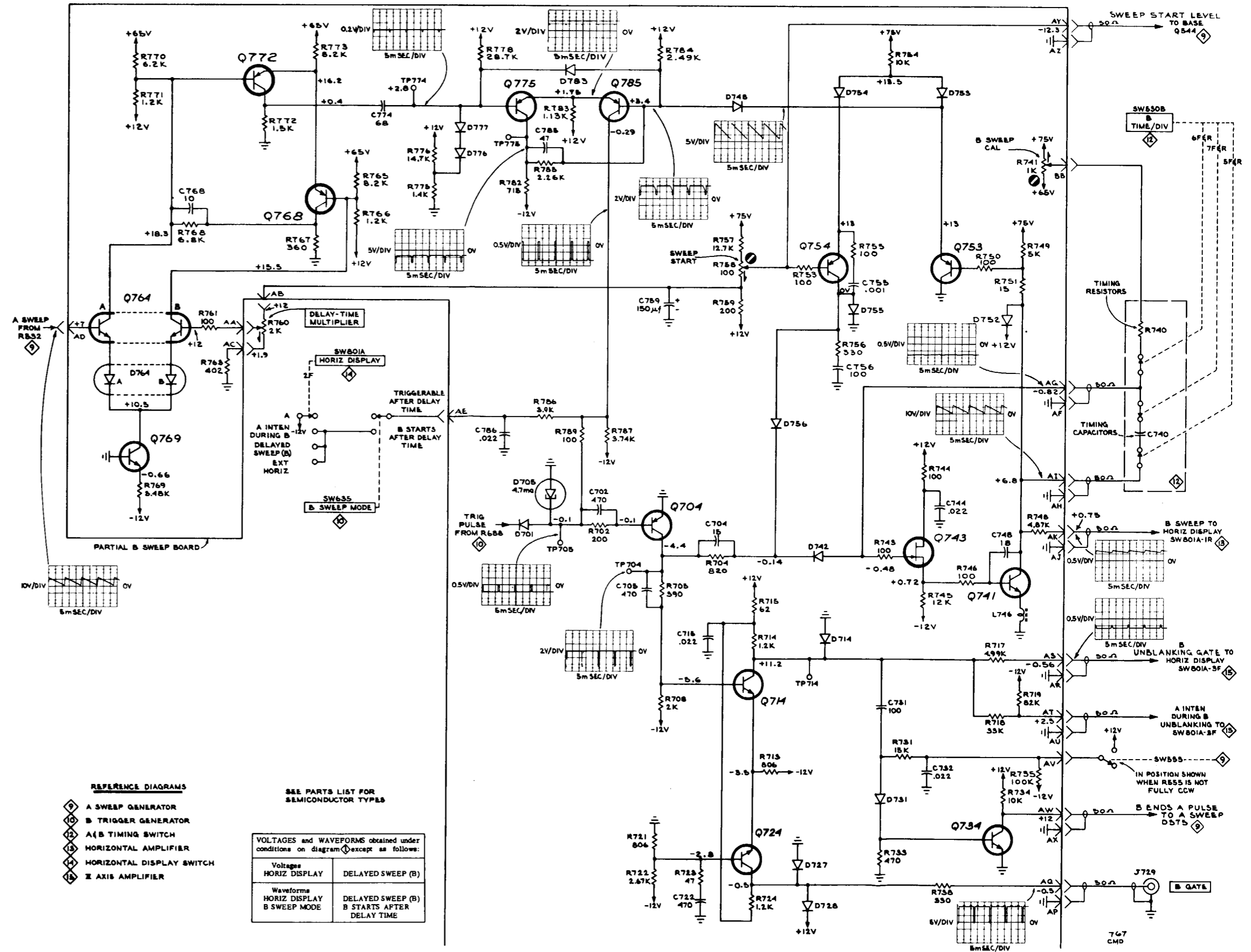
TYPE 453 OSCILLOSCOPE
