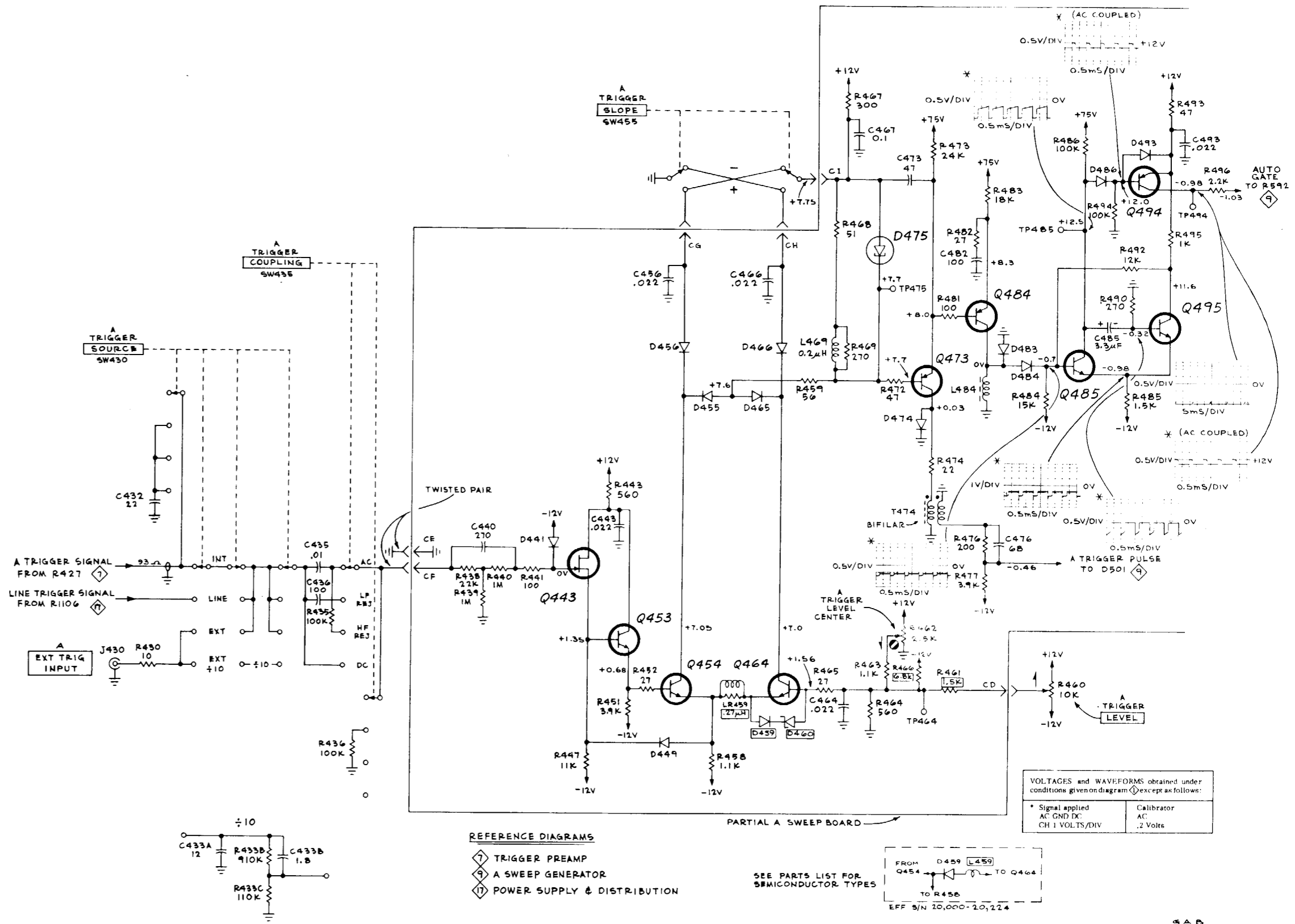
TYPE 453 OSCILLOSCOPE
