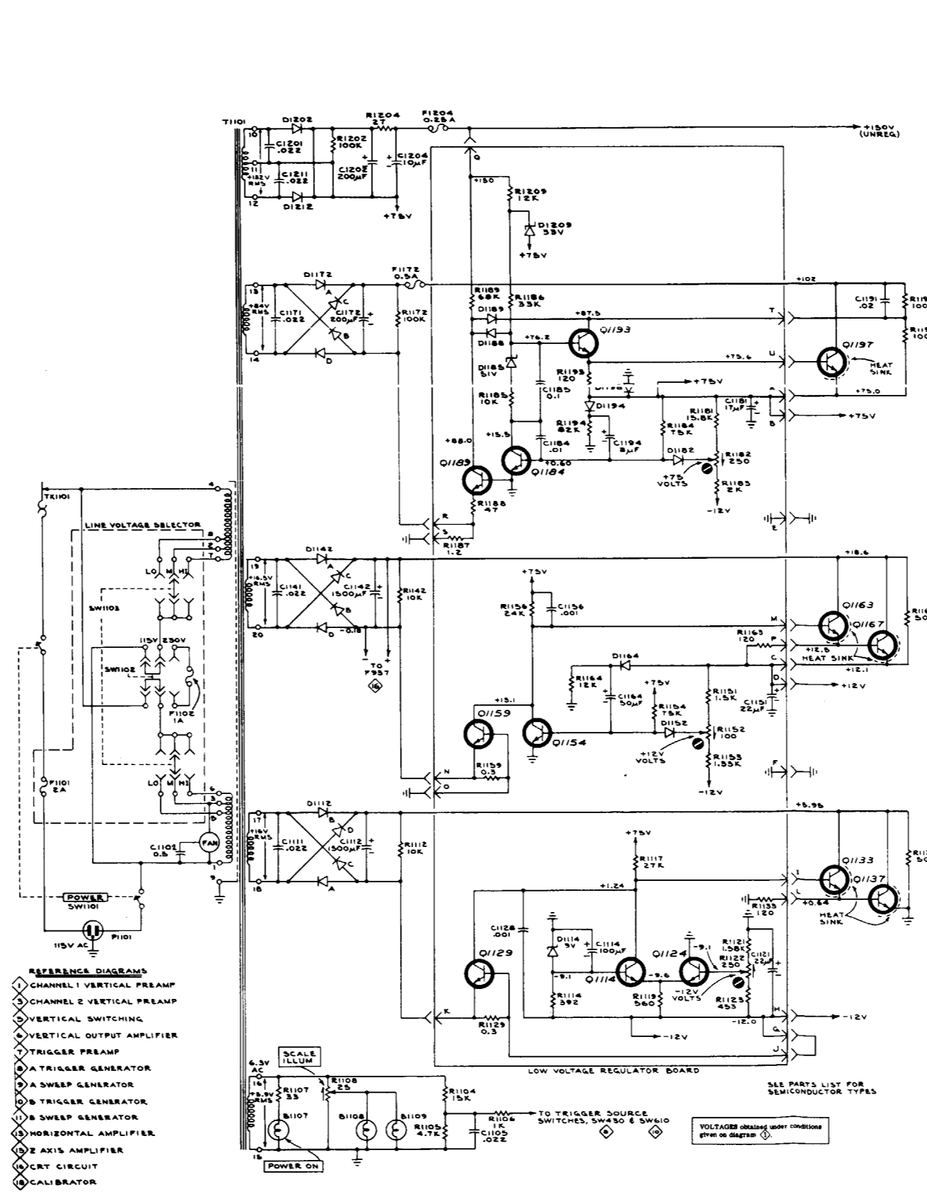
TYPE 453 OSCILLOSCOPE
