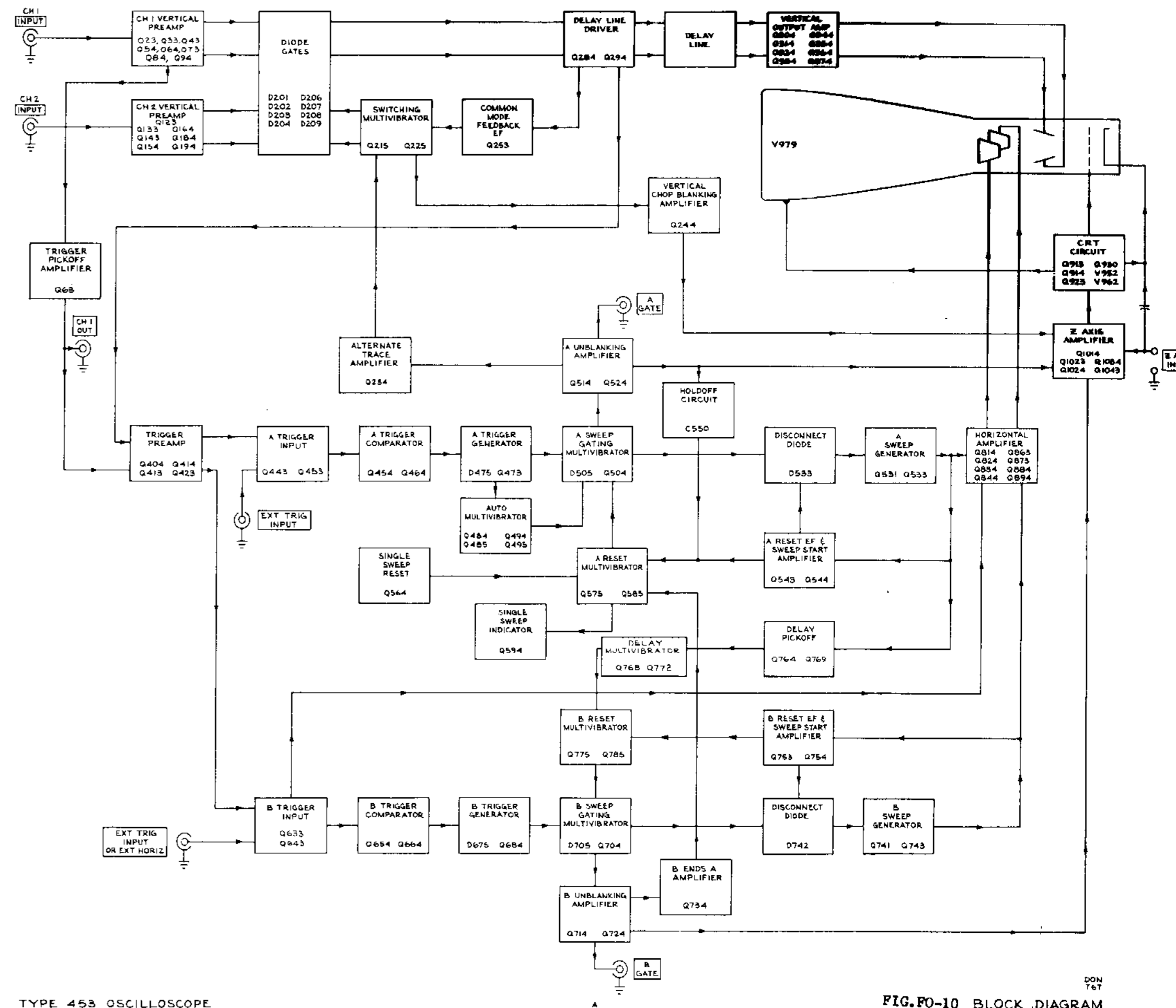
TYPE 453 OSCILLOSCOPE
